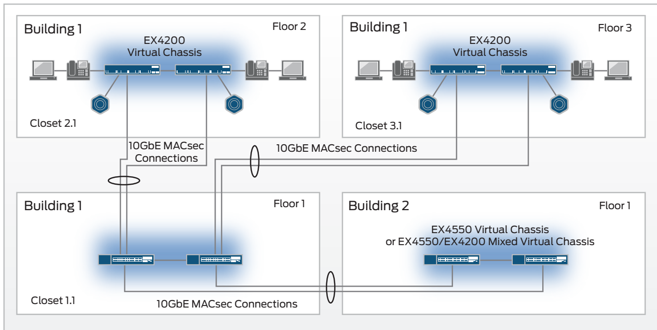
Figure 2: MACsec deployment with EX4200 and EX4550 switches.
