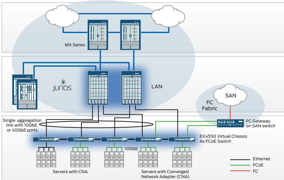
Figure 5: The EX4550 deployed as a data center FCoE transit switch in a top-of-rack Virtual Chassis configuration.
