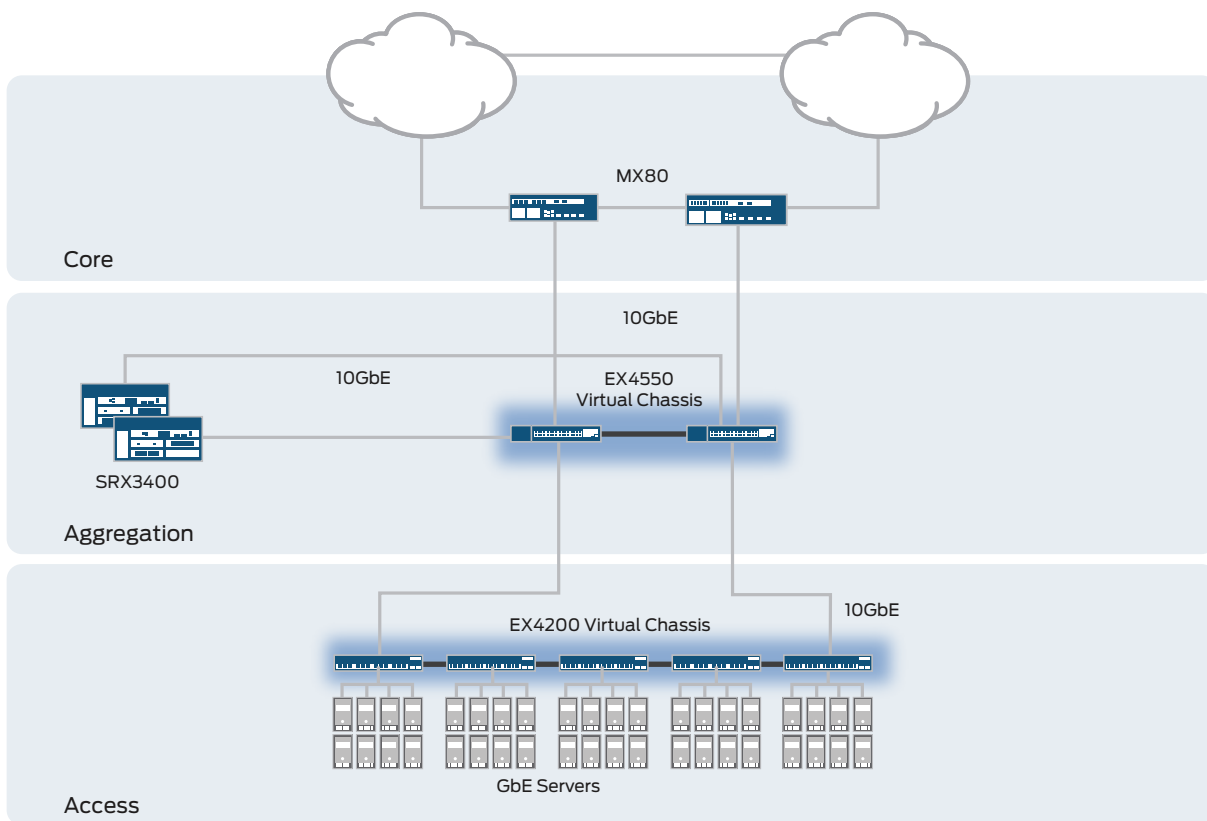
Figure 4: The EX4500 10GbE switch is ideal for small data center core deployments.
